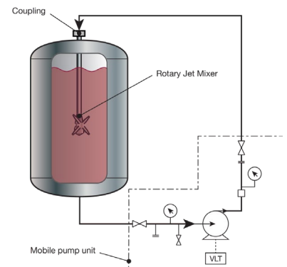
Rotary Jet Mixer Typical Installation
