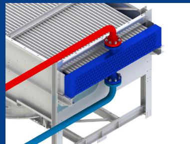
3. Match module process flanges to piping
