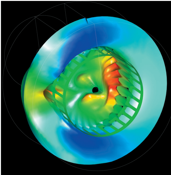
Velocity distribution in a Aalborg KBSA steam atomizing burner. Alfa Laval Aalborg engineers evaluate the combustion air distribution in a burner to increase its efficiency and reduce emission levels.
